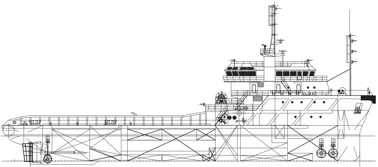
OUTBOARD PROFILE
